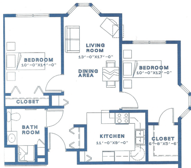
ONE BEDROOM PLAN C 835.34 Square Feet
