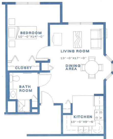
ONE BEDROOM PLAN B 675.66 Square Feet
