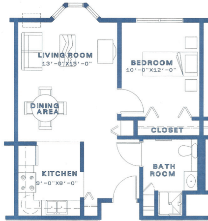
ONE BEDROOM PLAN A1/A2 603.63 Square Feet
